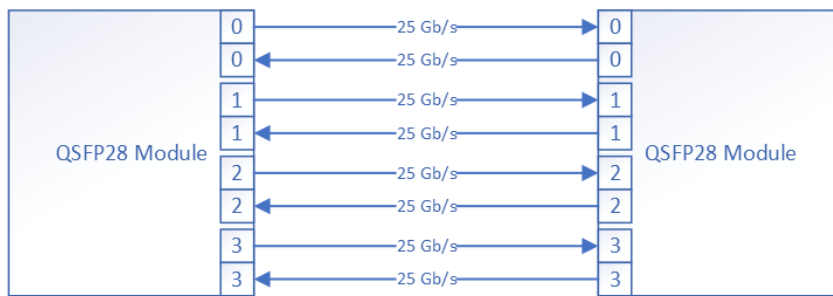
Figure 32.3. QSFP28 Interface (illustrative)
