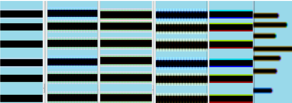
Figure 10.5. Periodic structure
