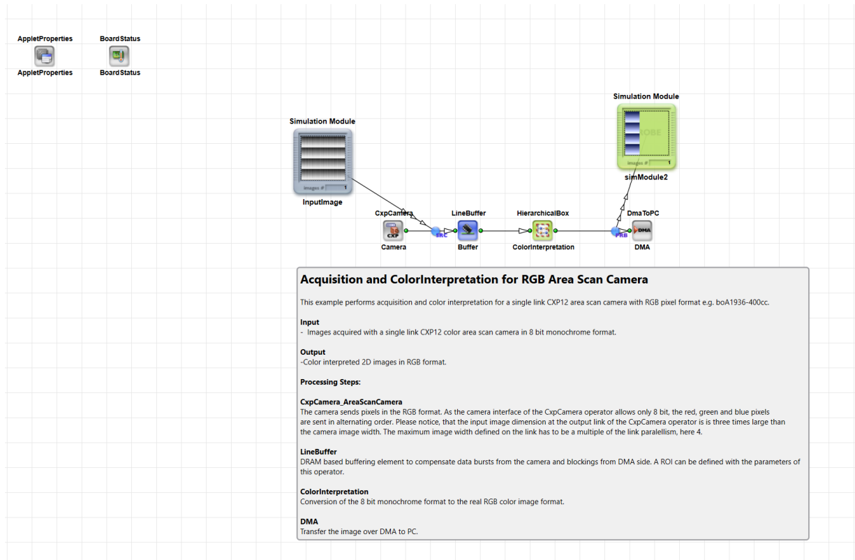
Figure 9.19. Basic Acquisition Example for Color Format Support on imaFlex Platform
