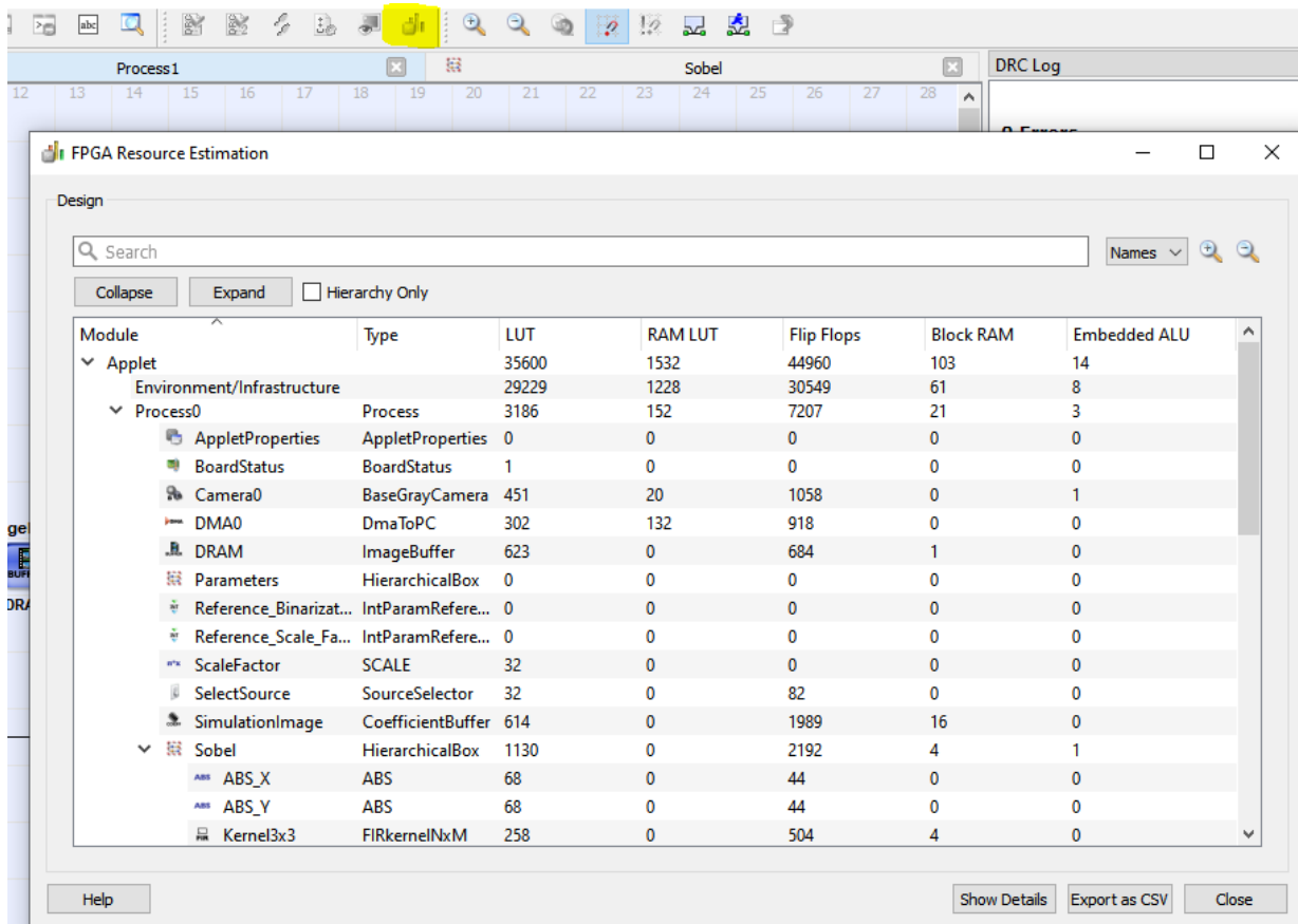
Figure 7.8. FPGA Resource Estimation
