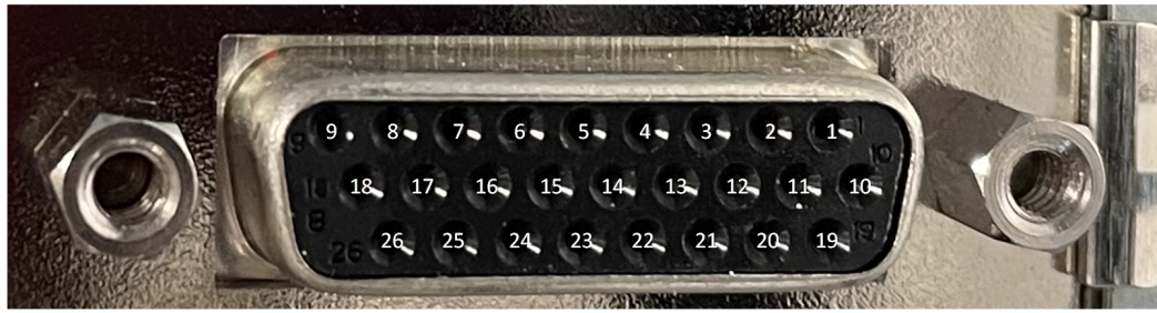
Figure 27.21. Front GPIO Connector of the imaFlex 2 Dual 100
