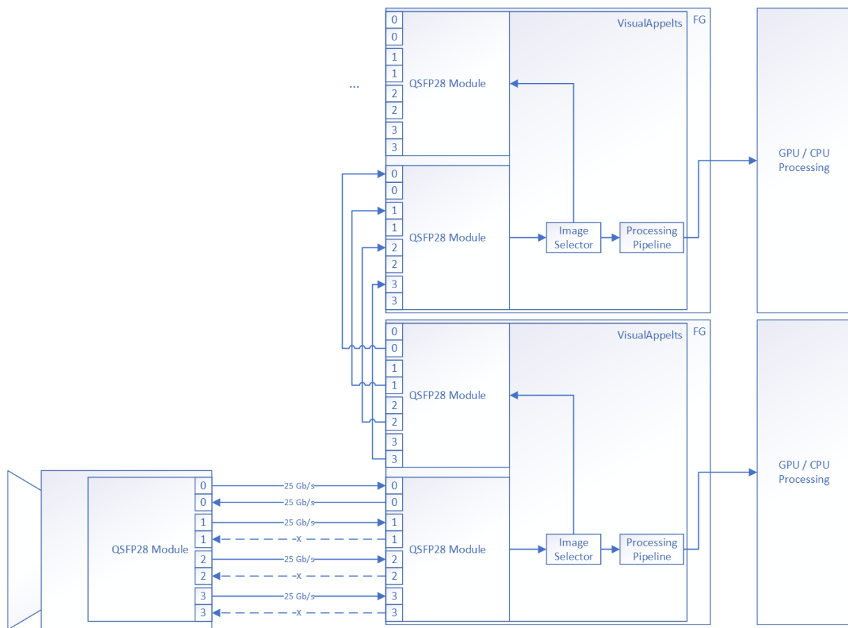
Figure 32.5. Data Forwarding Port Connection
