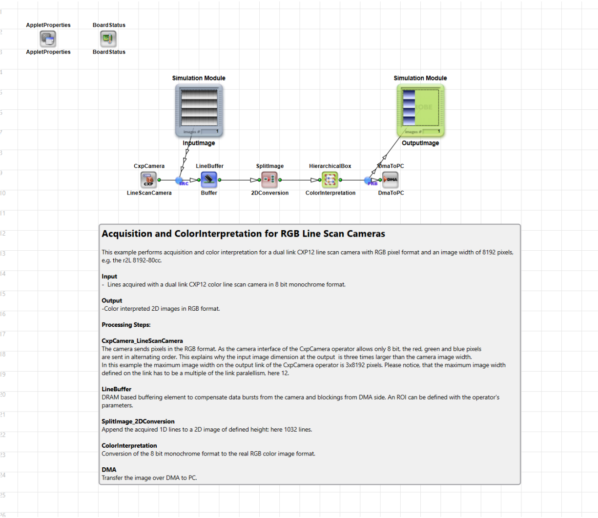
Figure 9.22. Basic Acquisition for RGB CoaxPress Line Scan Cameras on the imaFlex Frame Grabber
