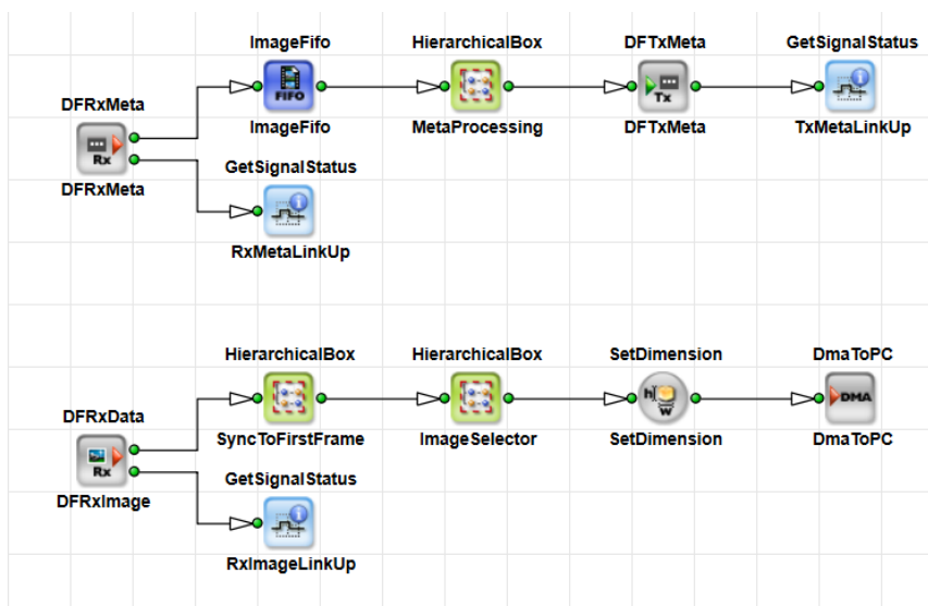
Figure 32.8. VA Design Example for an Endpoint Slave Master in a Data Forwarding Topology
