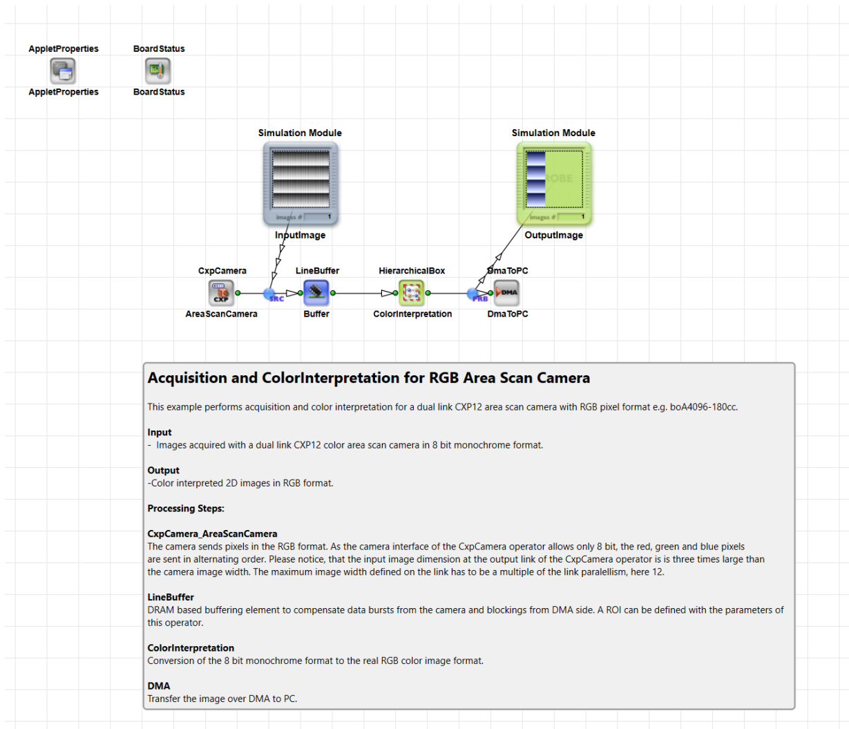
Figure 9.20. Basic Acquisition Example for Color Format Support on imaFlex Platform
