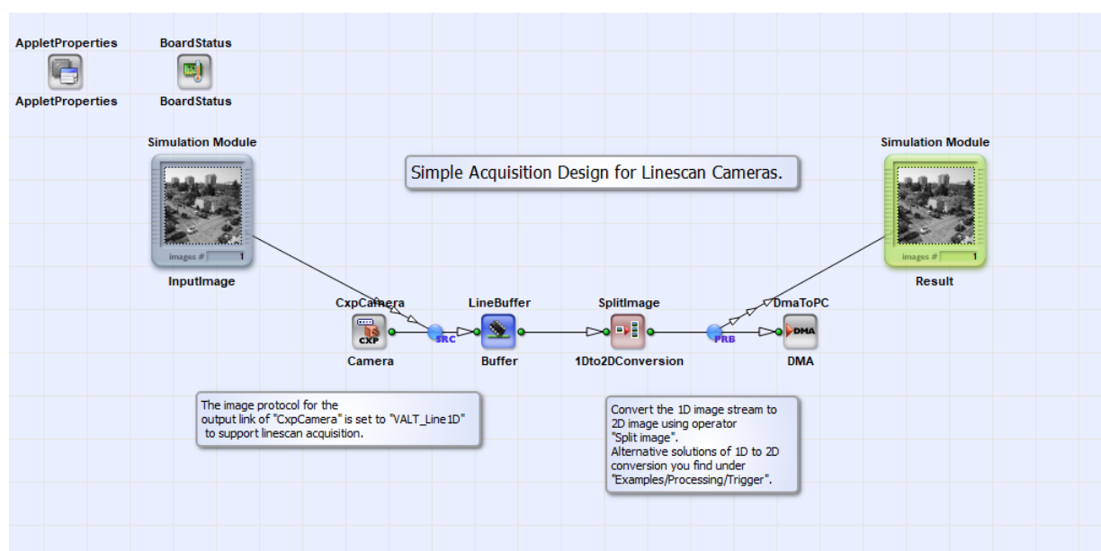
Figure 9.21. Basic Acquisition for Grayscale CoaxPress Line Scan Cameras on the imaFlex Frame Grabber
