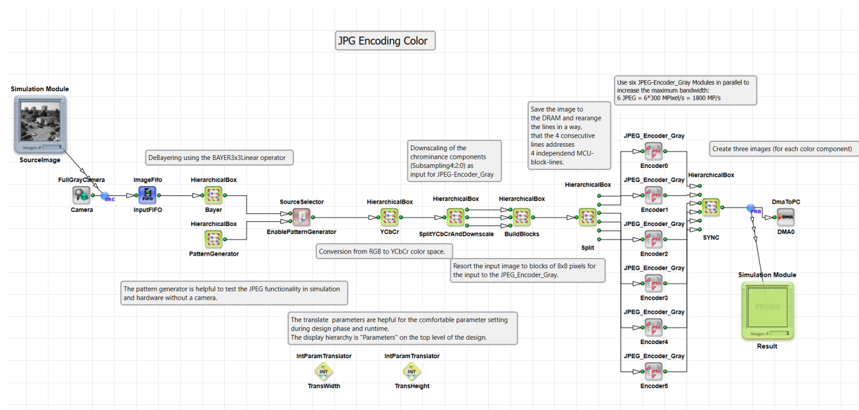
Figure 10.49. Basic design structure
